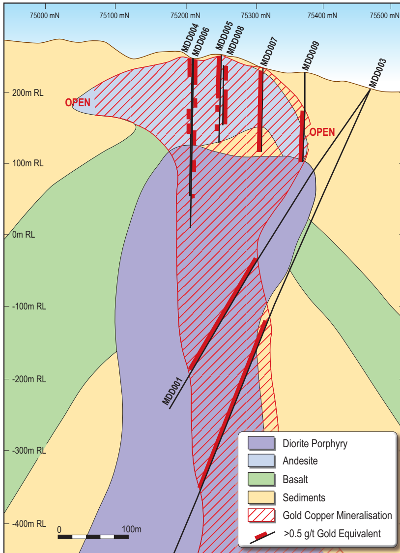
Schematic cross-section of Mapawa drilling results at 77880E showing intersections above 0.5g/t Au equivalent.
