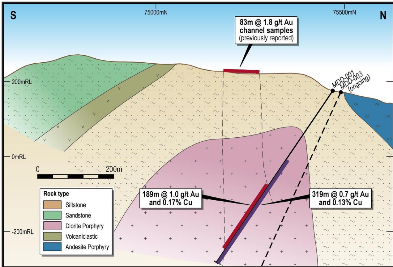
Section 77850mE showing MDD001 drilling result and interpreted geology.
